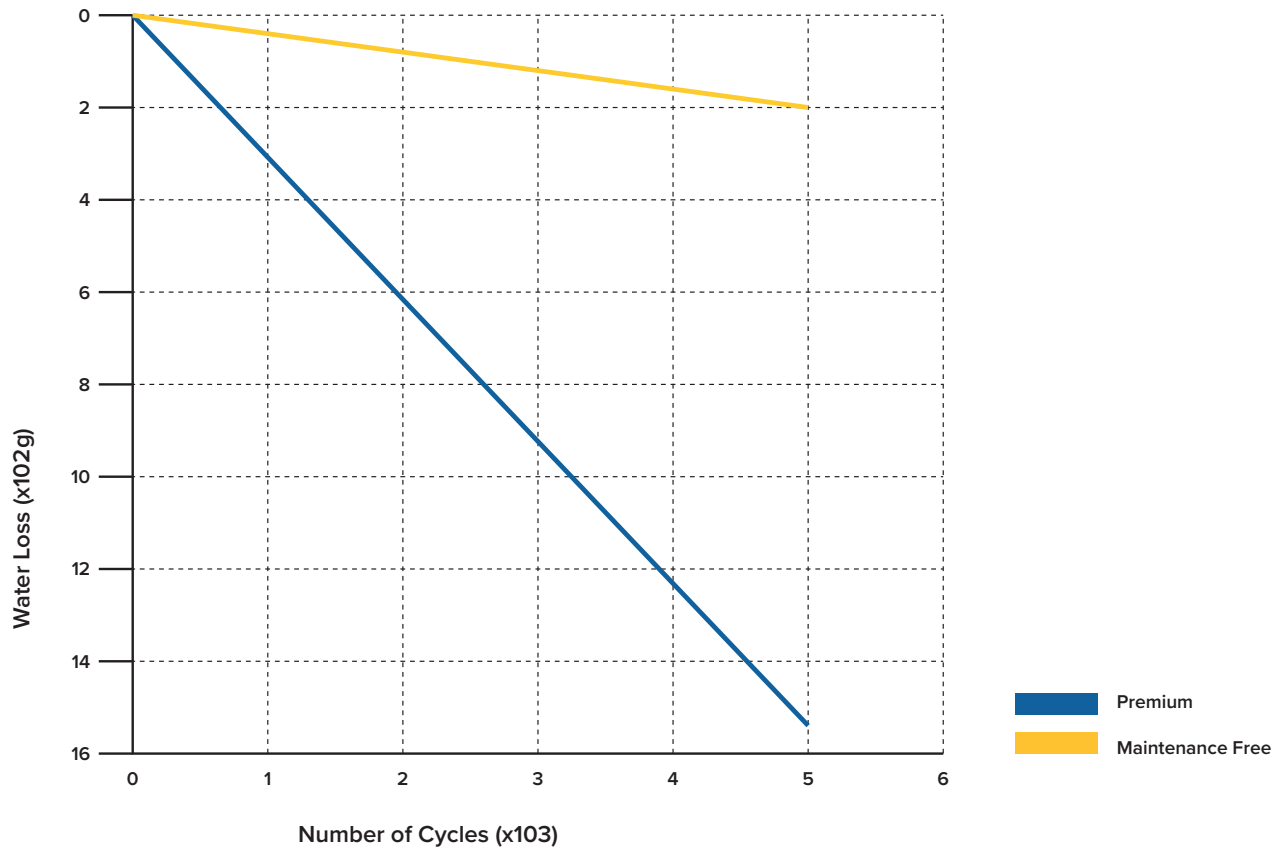
Graphic Water Loss Rate Premium - Maintenance Free
