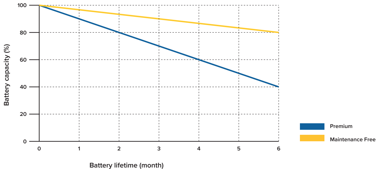
Graphic Self Discharge Premium - Maintenance Free (Temperature test 30°C)
